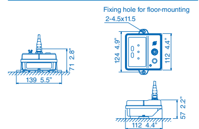
PG-700 Main Unit (Floor Mount)
