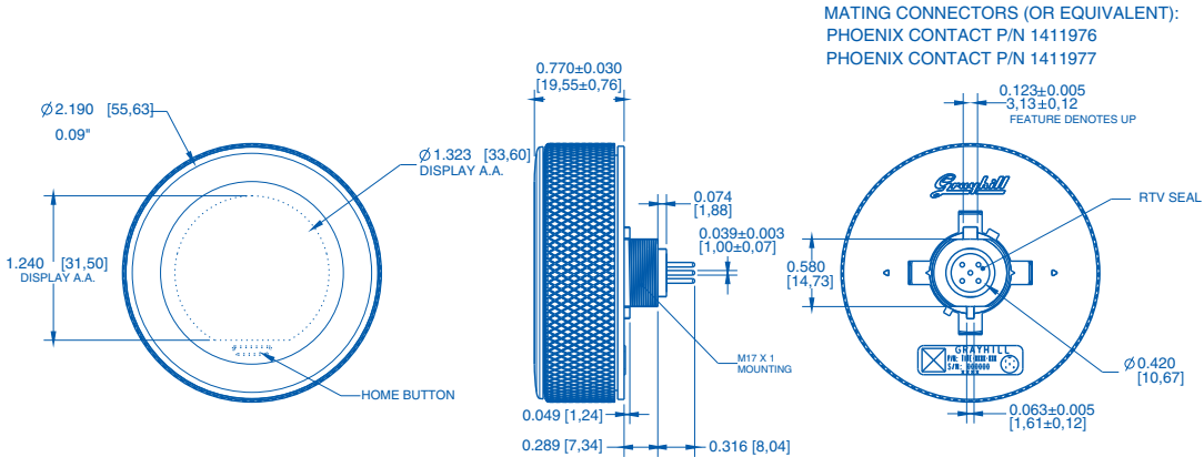
Touch Encoder Unit TEU001B/S (option, U.S. and Canada only) 0.12 kg 0.26 lb
