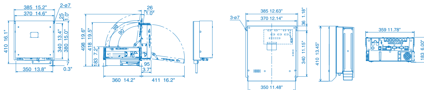
Processor Unit RPU-025
