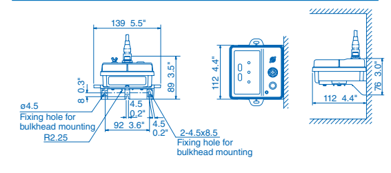
PG-700 Main Unit (Bulkhead Mount)
