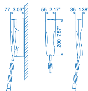
Handset HS-2003
