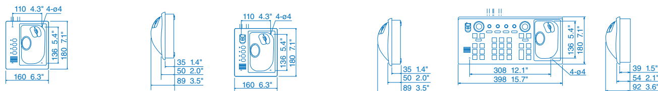
Trackball Control Unit RCU-016
