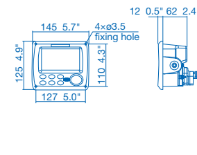
Display Unit FA-170I
